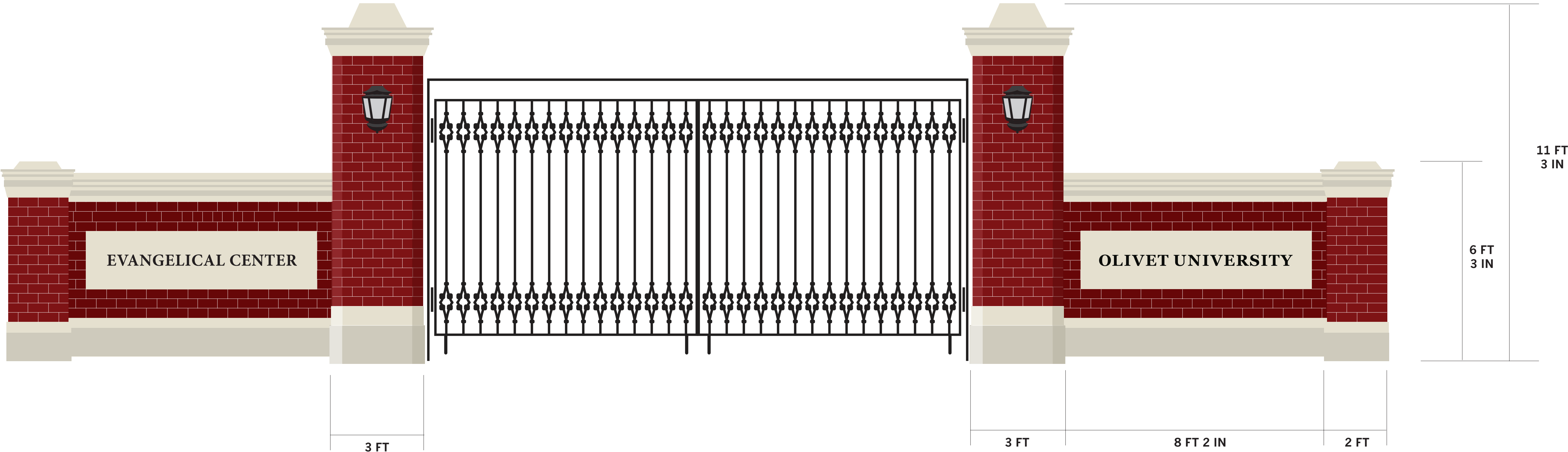
Front View
